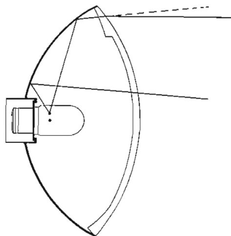
PRISMATIC ACTION OF DIPPED BEAM
