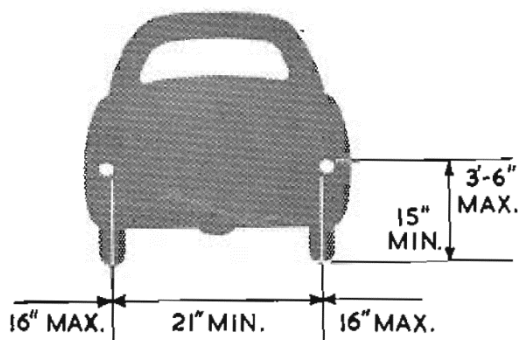
Reflectors on Private Cars, Goods Vehicles under 30 cwt., Three-wheel Cars and Trailers must not be more than 30 inches from the extreme rear.
