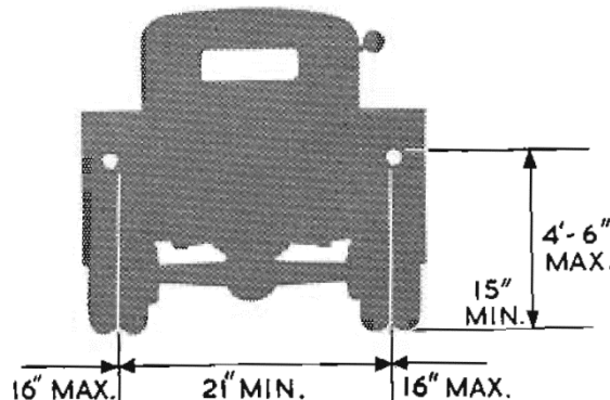
Reflectors on Goods Vehicles over 30 cwt. must not be more than 30 inches from the extreme rear.
