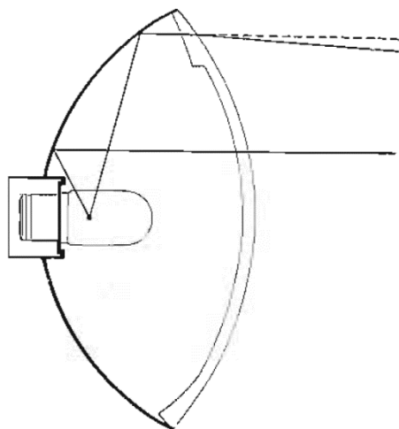
PRISMATIC ACTION OF MAIN BEAM
