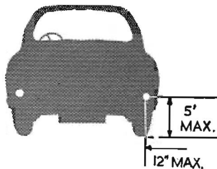
Sidelamps — maximum bulb rating 7 watts.
